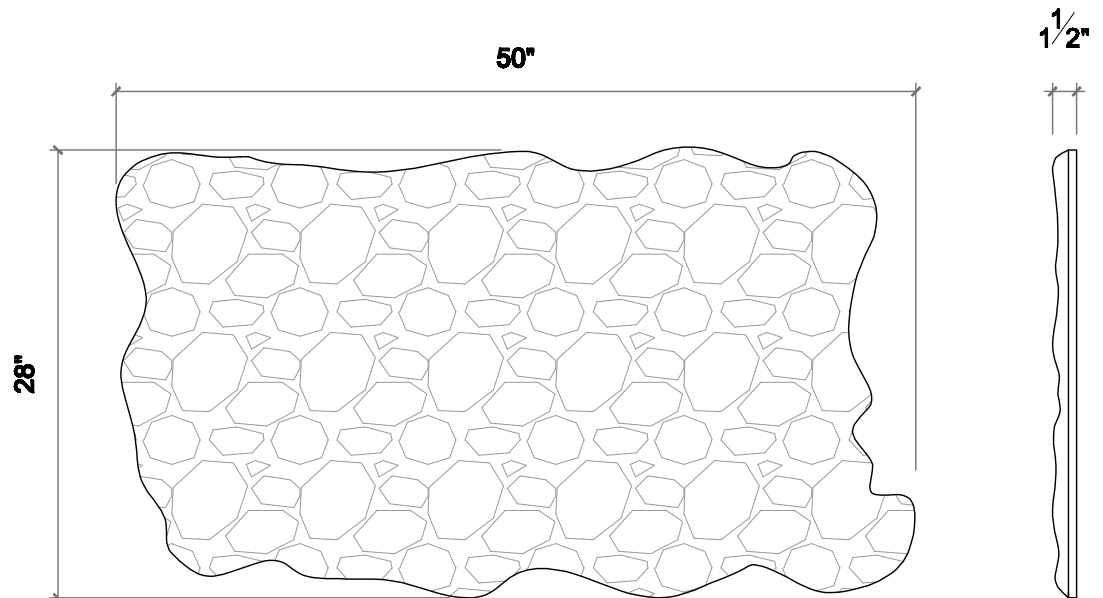
Front View
