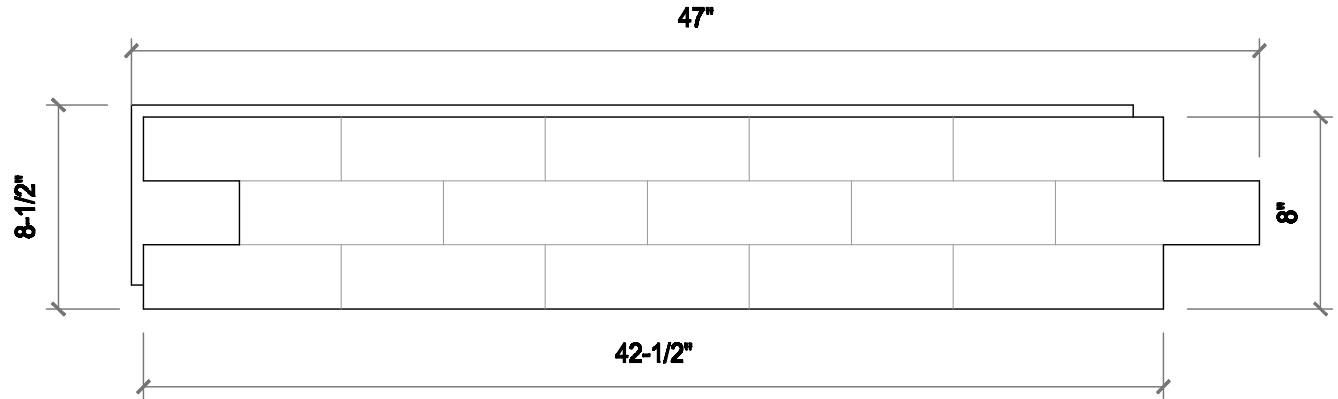
Front View
